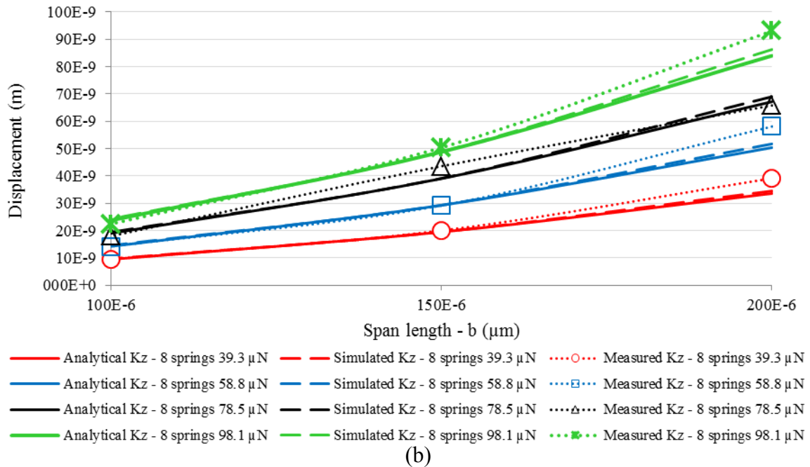
Figure 6-3: Spring/proof mass displacement comparison (a) analytical vs. measured (b) simulated vs. measured
