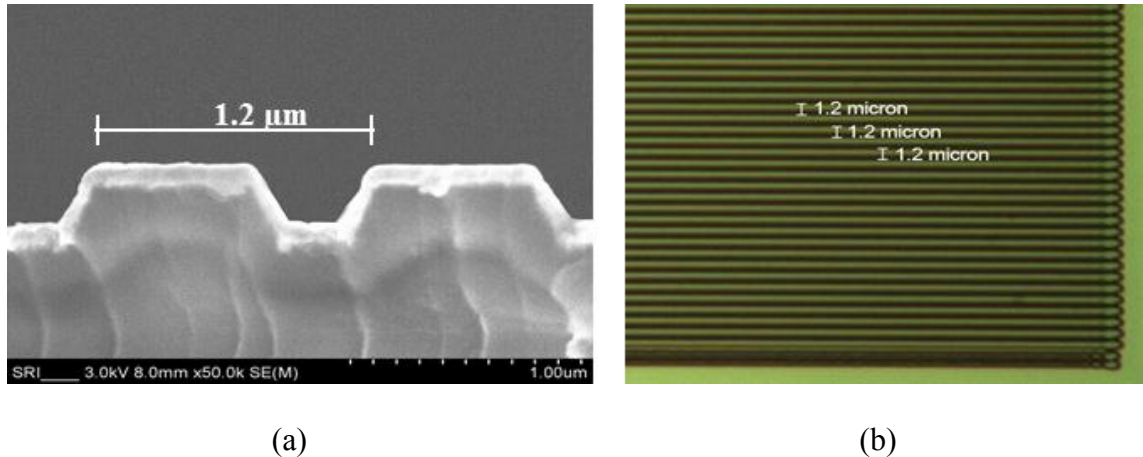
Figure 4-5: SEM image of the SW gratings etched into the glass substrate coated with Au/Pd to dissipate charging (a) cross-section view (b) microscope view of the SW gratings
