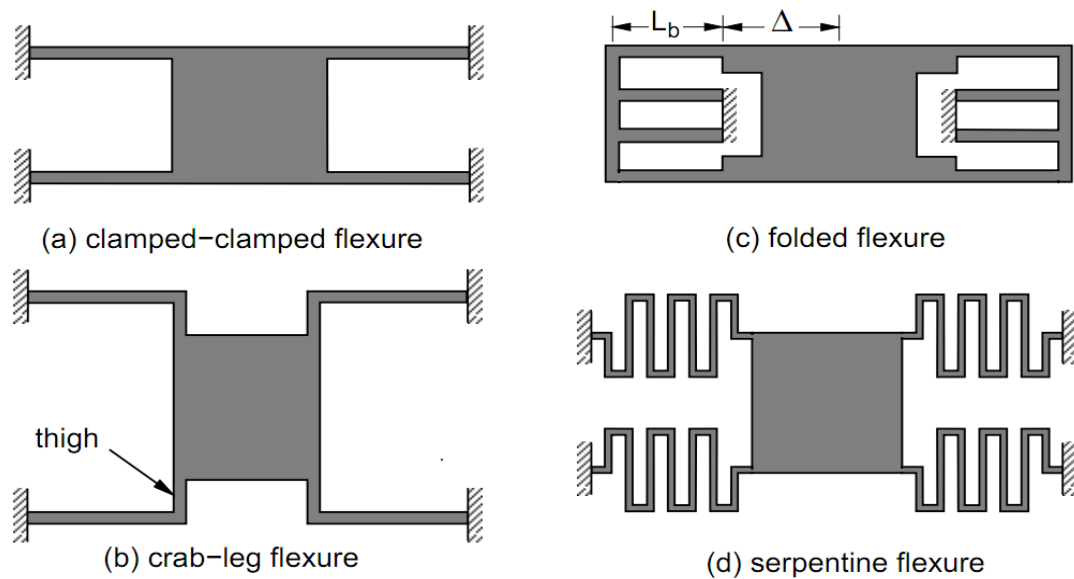
Figure 3-11: Various spring designs (a) fixed-fixed flexure (b) crab-leg flexure (c) folded flexure (d) serpentine flexure [56]
